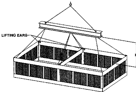
Figure 2b – 6m (20'), 7.3m (24'), 8.6m (28') & 11m (36') Long Bottom Section, Models AT/UT/USS 420-124 through 420-924, 420-136 through 420-936 and 424-024 through 424-936.
