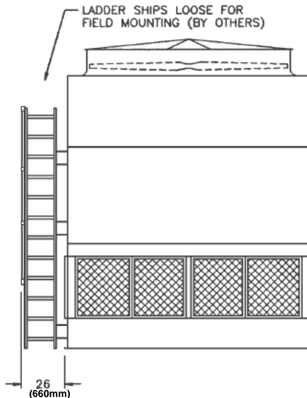
Figure 23A - End View of Ladder Assembly
