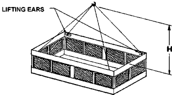
Figure 2a -3.6m (12') and 5.5m (18') Long Bottom Section, Models 220-112 through 220-912, 220-118 through 220-918 and 224-018 through 224-918
