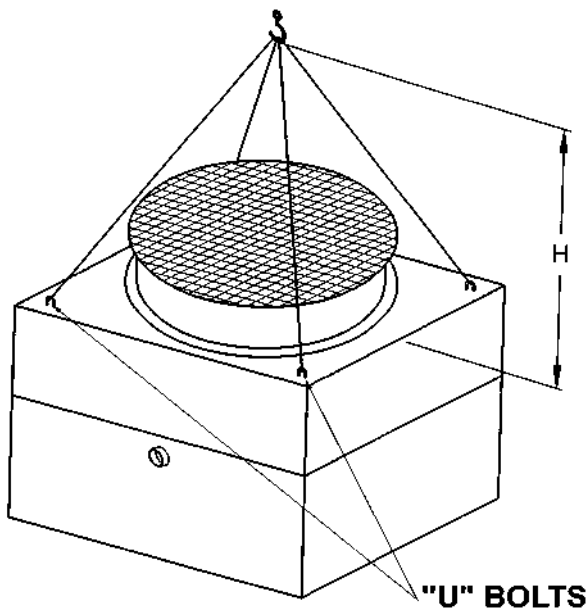
Figure 9 - Top Section(s)
