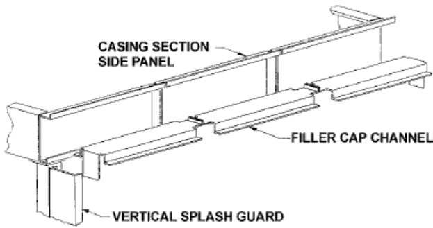
Figure 14- Filler Cap Channel Assembly.
