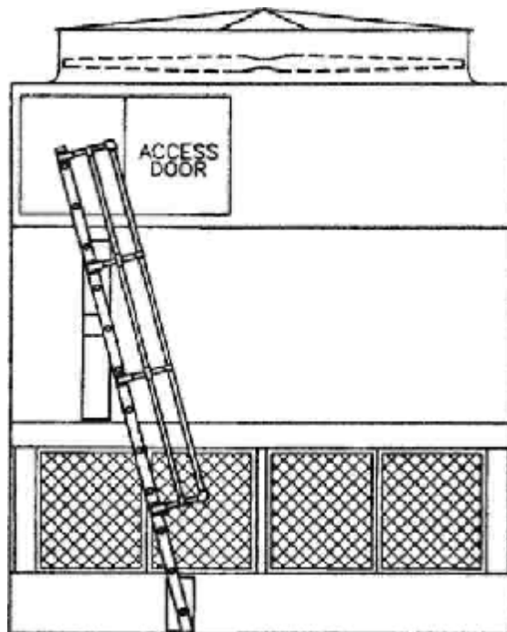
Figure 23B - Side View of Ladder Assembly
