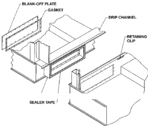
Figure 6 - Optional Blank-Off Plate on the Equalizer Flume
