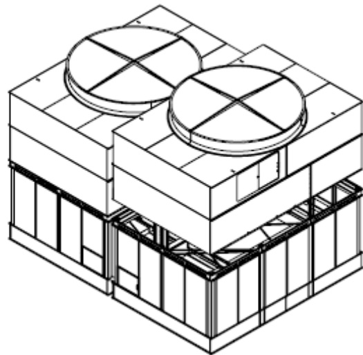
Figure 13 - Mating Upper Section to Bottom Section.
