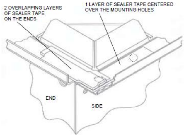
Figure 7 - Sealer Tape on flange of Bottom Section.
