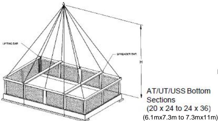
Figure 12 - Proper Rigging Method for Extended Lifts.
