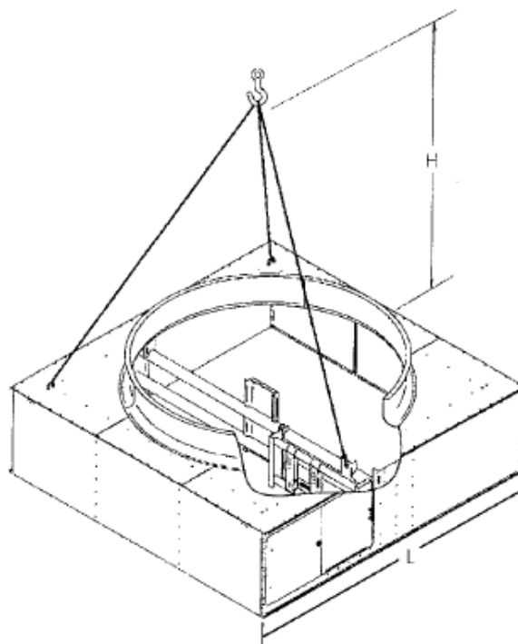
Figure 10 - Three Point Rigging of the Fan Section
