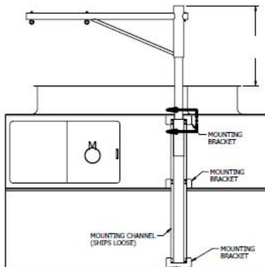
Figure 20 - Dual Point Davit Arrangement.
