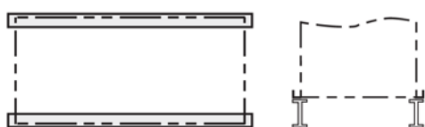
Figure 1 - Steel Support (3', 4', 8.5', 10' and 12' wide models)
