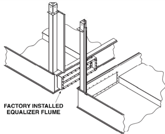
Figure 6 - Equalizer Flume Rigging Detail, 12' Wide Models
