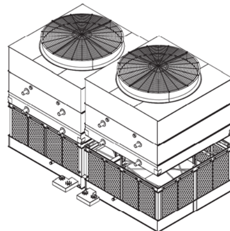
Figure 16 - Mating Upper Section to Basin Section
