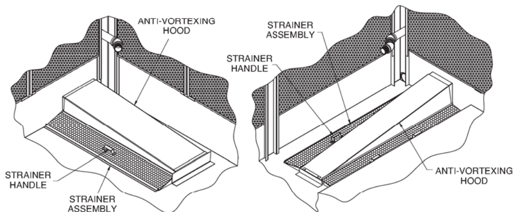
Figure 31 - Strainer Location
