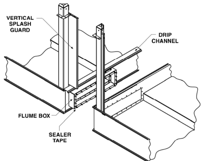
Figure 5 - Equalizer Flume Connection, 12' Wide Models
