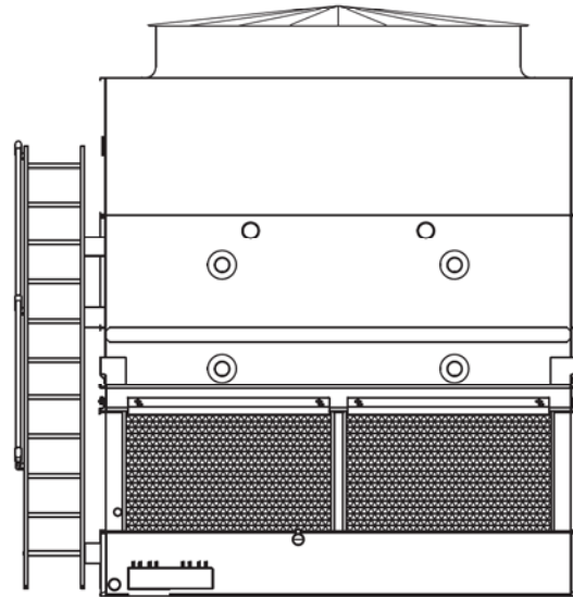
Figure 23 - End View of Ladder Assembly
