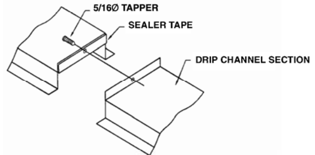
Figure 9 - Drip Channel Assembly
