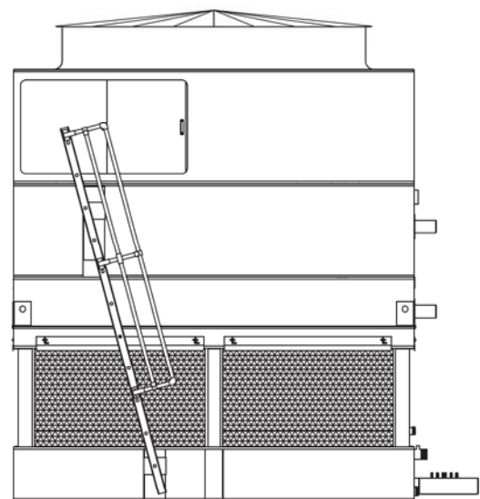
Figure 24 - Side View of Ladder Assembly
